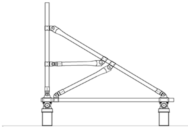
Example of RoofScreen NC5 Frame Configuration
