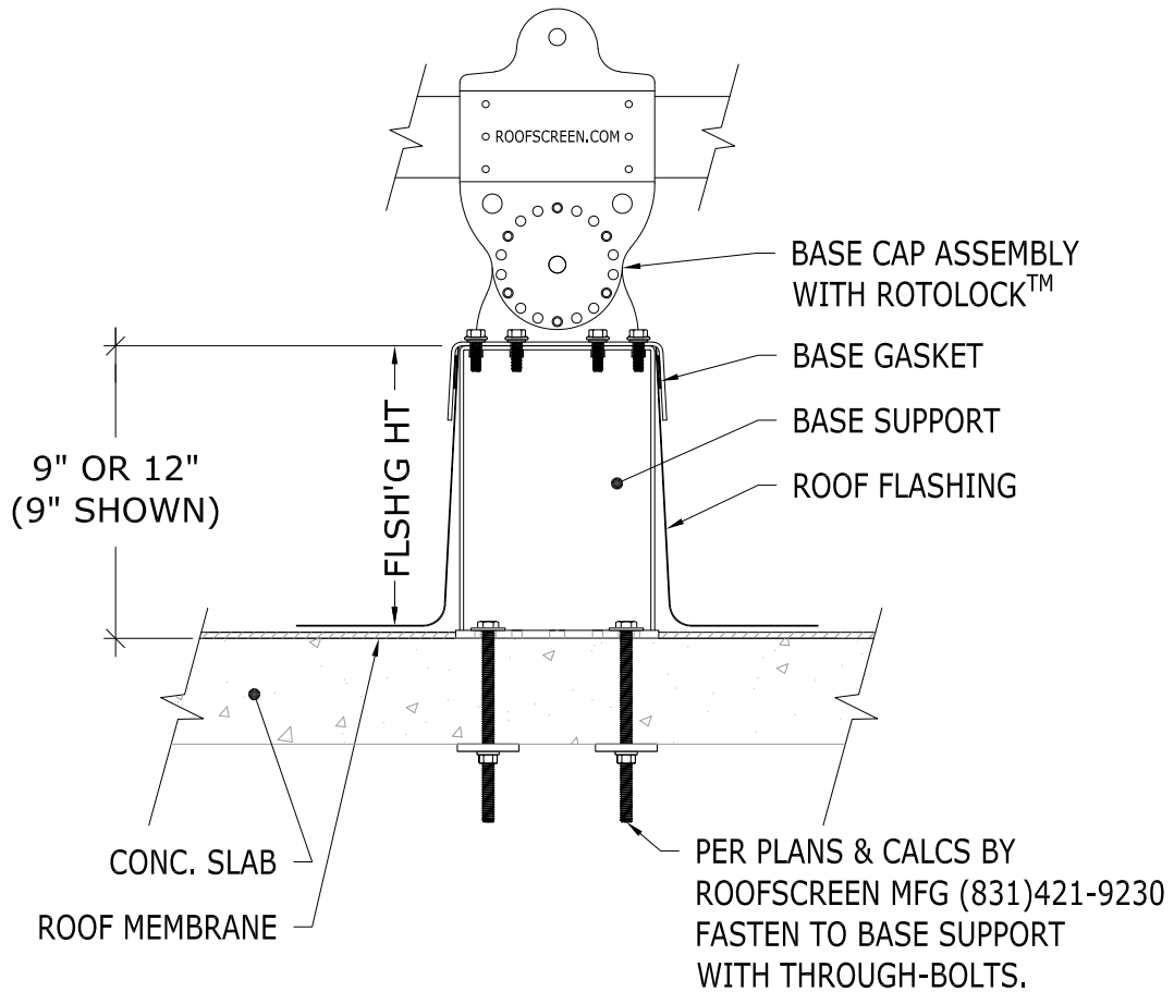
STRUCTURAL CONCRETE THROUGH-BOLTS - NO INSULATION - NO EXTENSION
