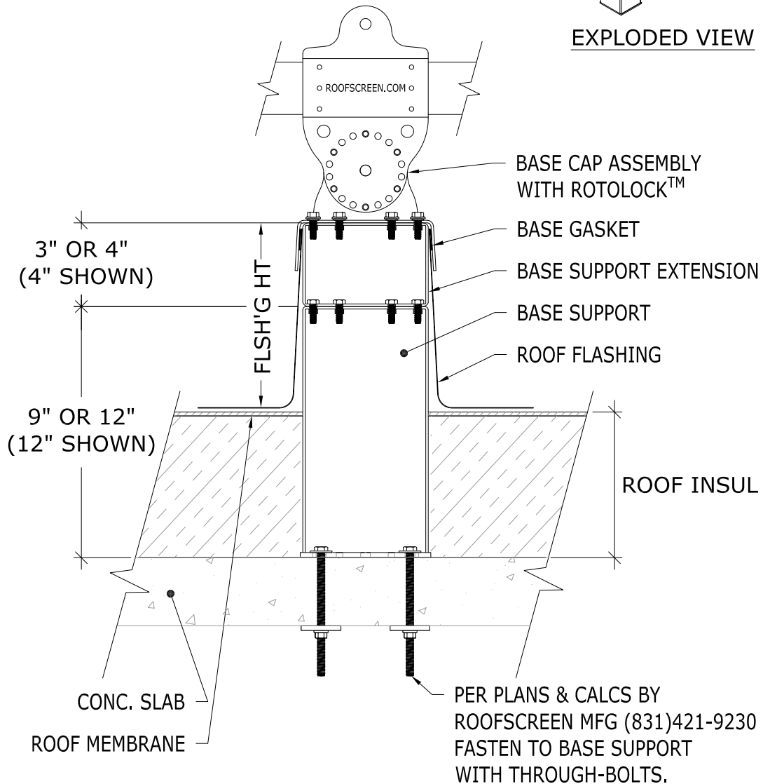
STRUCTURAL CONCRETE THROUGH-BOLTS - WITH INSULATION - WITH EXTENSION
