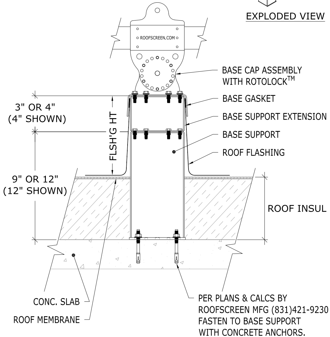
STRUCTURAL CONCRETE CONCRETE ANCHORS - WITH INSULATION - WITH EXTENSION
