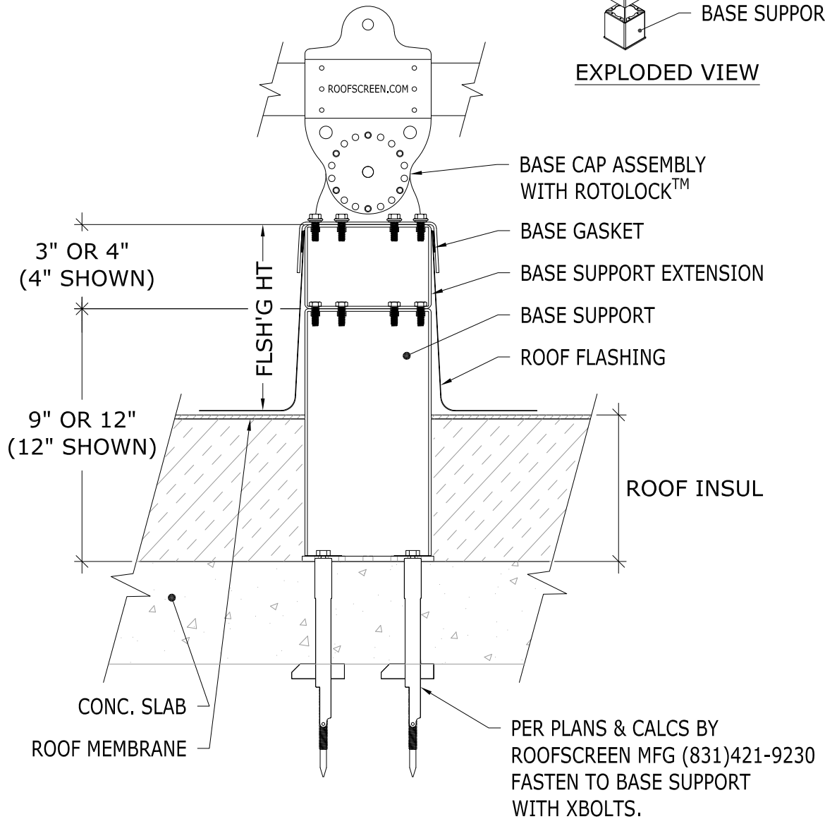
STRUCTURAL CONCRETE XBOLTS - WITH INSULATION - WITH EXTENSION
