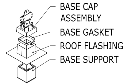
EXPLODED VIEW
