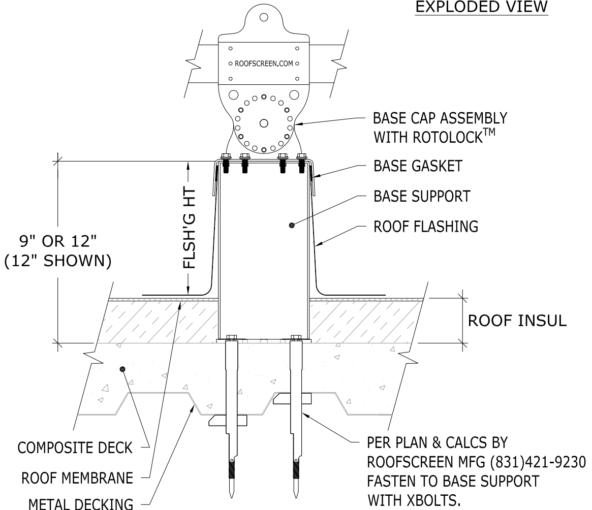
EXPLODED VIEW
