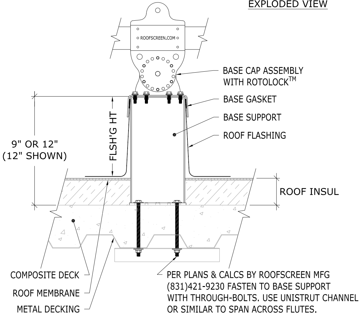
EXPLODED VIEW
