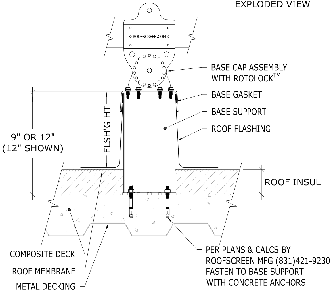
EXPLODED VIEW
