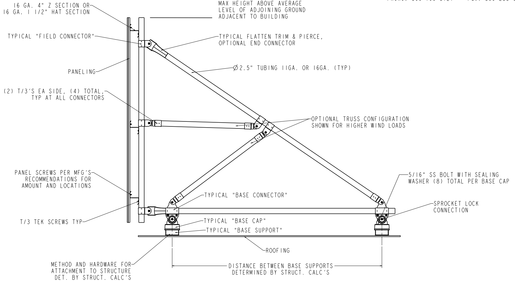
TYPICAL ROOFSCREEN TUBE FRAME
