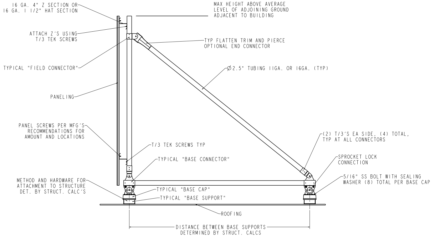
TYPICAL ROOFSCREEN NO CANTILEVER FRAME
