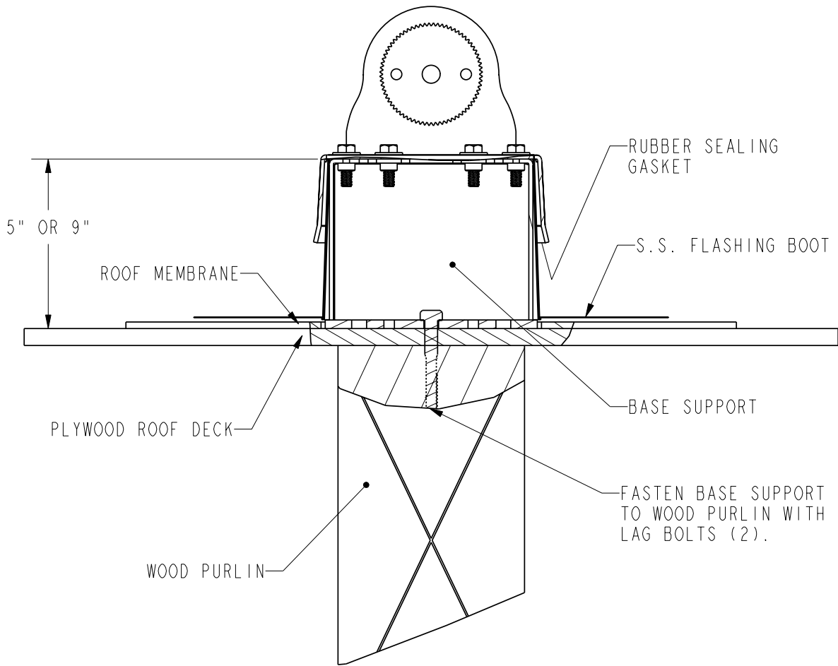
SECTION B-B
